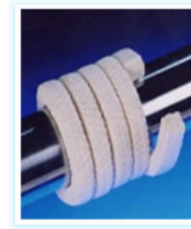
Pure PTFE Teflon® Packing – With Oil Lubricant
